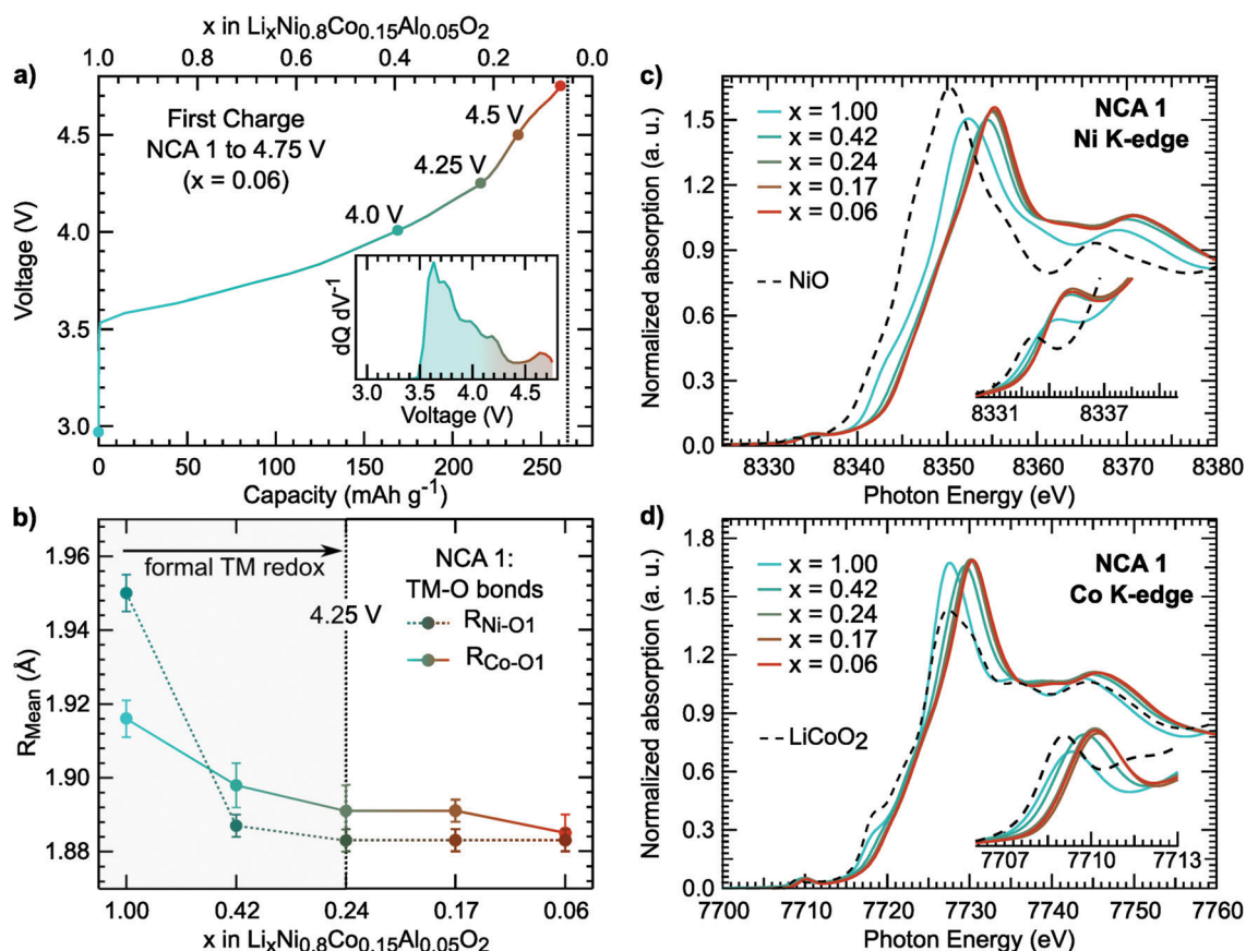
Fig. 2 (a) Electrochemical profile of first charge and dQ \, dV^{-1} (inset) including the cutoff voltages of the selected NCA 1 electrodes used for X-ray spectroscopy measurements. (b) Ni–O1 and Co–O1 bond lengths derived from EXAFS fits. Example fits for the Ni and Co K-edge EXAFS are given in Fig. S1 (ESI†). The average Ni–O bond length of the pristine sample is similar to previously reported \text{LiNiO}_2 61 (c and d) XANES measurements of the Ni and Co K-edges including \text{NiO} ( \text{Ni}^{2+} ) and \text{LiCoO}_2 ( \text{Co}^{3+} ) references.
