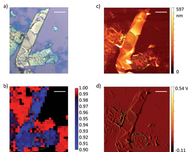
Fig. 4 Graphite and graphene flakes on SiO 2 (300 nm)/Si. (a) shows the optical microscope image of that area, and (b) shows the coefficient of determination R^2 of the Raman 2D band fit with values considered as graphite in blue, as graphene in red and the substrate in black. (c) and (d) depict the AFM measured height and error signal respectively. Scale bars are 5 \mu m.
