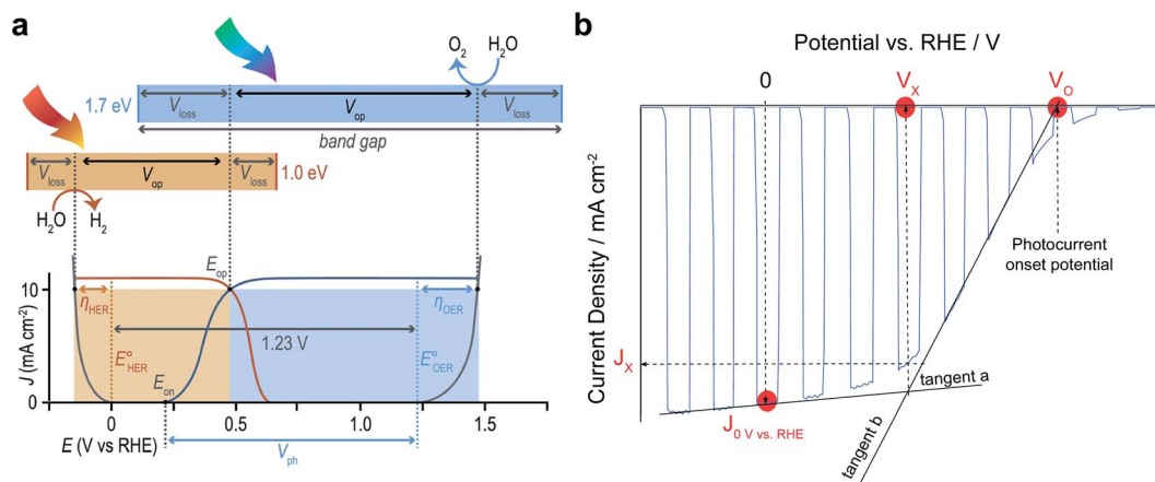
Fig. 12 (a) Schematic relating band gaps and photovoltages for an idealised two-absorber tandem photoelectrolysis device in which the anode is the top absorber. Free energy losses in each absorber ( V_{\text{loss}} ) and catalytic overpotentials for each half-reaction ( \eta ) are fundamental loss pathways. Current density–potential curves for electrocatalysts (grey) and an idealised PEC photoanode (blue) and photocathode (orange) are shown with their relative power contributions (shaded areas) in an ideal tandem operating at E_{\text{op}} being the intersection of the two J – V curves. Reprinted from ref. 6 with permission from Elsevier. (b) Useful benchmark parameters in a current density–potential ( J – V ) curve of typical OPEC cells showing the current density at 0 \text{ V vs. RHE} , the photocurrent J_x at the cross-over potential V_x and the photocurrent onset potential V_0 . For simplicity, a photocathode J – V curve was chosen.
