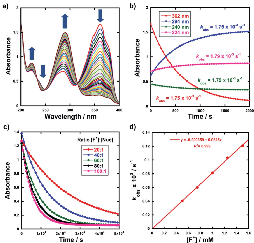
Fig. 2 (a) UV-vis spectra during the reaction of 1d (0.05 mM) with Selectfluor TM (in \text{CH}_3\text{CN} at 25^\circ\text{C} ), each spectrum acquired at 30 s intervals. The shoulders at 350 nm are artefacts that correspond to the spectrophotometer switching from UV to VIS lamps. (b) Exponential behaviour at 4 different wavelengths. (c) Representative exponential decays of absorbance with different concentrations of \text{F}^+ . (d) Representative correlation of k_{\text{obs}} with [\text{F}^+] .
