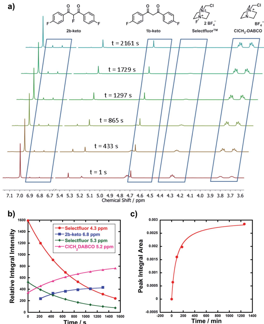
Fig. 3 (a) Time-arrayed ^1\text{H} NMR experiment with 1b and Selectfluor TM 3 under pseudo-first order conditions, with a 10-fold excess of 1b . Spectra were acquired at 3.6 min intervals and illustrative spectra from this time-course are shown above. Key signals are indicated with their associated structures. The enol form of 1b corresponds to the peak at 7 ppm. Peaks at 5.3 and 5.2 ppm correspond to disappearance of Selectfluor TM 3 and appearance of its defluorinated product, respectively. (b) Reaction profile by ^1\text{H} NMR (reaction of 1b with Selectfluor TM 3 ). (c) Reaction profile for LCMS analysis of the reaction between diOMe substrate 1d and Cl 2 -NFPy BF 4 − 8b under bimolecular reaction conditions ([Nuc] = [F + ] = 3 mM).
