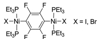
Scheme 4 Dinuclear product [\text{trans-NiX}(\text{PEt}_3)_2]_2(\mu\text{-2,3,5,6-C}_6\text{F}_4) .
