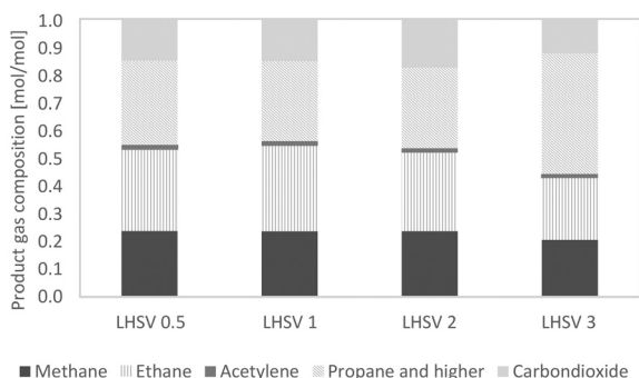
Fig. 5 Composition of gaseous products dependent on LHSV [ \text{h}^{-1} ] after 36 h of experiment.
