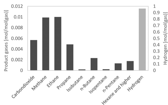
Fig. 6 Gas analysis according to DIN 5166, for the experiment at the LHSV of 0.5 \text{ h}^{-1} .
