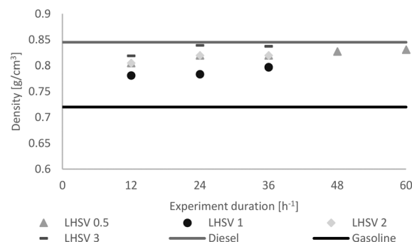
Fig. 8 Distribution of the density of the hydrocarbon product phase dependent on the LHSV [ \text{h}^{-1} ] compared to the minimum of gasoline and the maximum of diesel, according to EN228 (ref. 35) and EN590. 34
