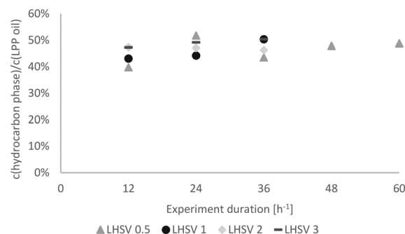
Fig. 7 Carbon yield in the hydrocarbon product phase over the experiment duration dependent on the LHSV [ \text{h}^{-1} ].
