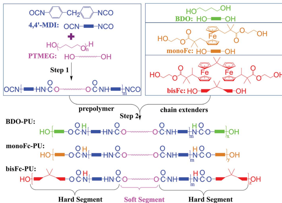
Scheme 1 Synthetic routes for polyurethanes with different chain extenders: 1,4-butanediol (BDO), 1,1'-bis[2-(β-hydroxyethyl)ester-2-methyl-propyl]ferrocene (monoFc), and 6,6'-bis[1-methyl-2-(β-hydroxyethyl)ester-2-methyl-propyl]bisferrocene (bisFc).
