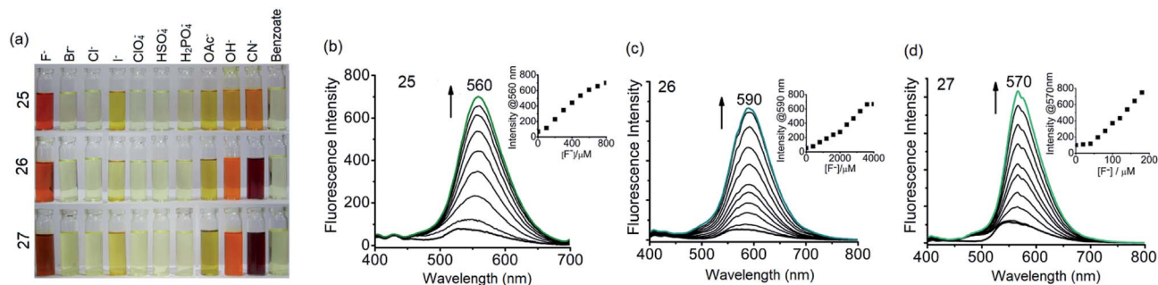
Fig. 14 (a) Chromogenic response of 25 – 27 ( 10.0 \times 10^{-3} M in dry tetrahydrofuran) in the presence of 20 equivalents of various anions, (b) PL spectra of 25 with TBAF (0 to 40 equivalents), (c) PL spectra of 26 with TBAF (0 to 200 equivalents) and (d) PL spectra of 27 with TBAF (0 to 10 equivalents). The insets in b–d show emission intensity versus concentration of TBAF. Reproduced from ref. 63 with permission. Copyright© 2016, Springer Nature.
