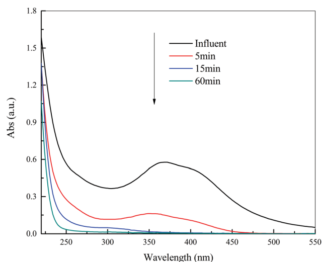
Fig. 3 UV-Vis spectra of DDNP industrial wastewater as a function of time. Condition: temperature of 90\text{ }^{\circ}\text{C} , PS dosage of 20.0\text{ g L}^{-1} and initial pH of 2.0.
