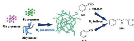
Scheme 1 Schematic of the synthesis of PtMo WNWs and its catalytic application in the DBA synthesis from reductive amination of either BzH or BzN.
