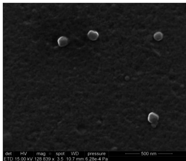
Fig. 3 SEM image of the histamine nanoMIPs.
