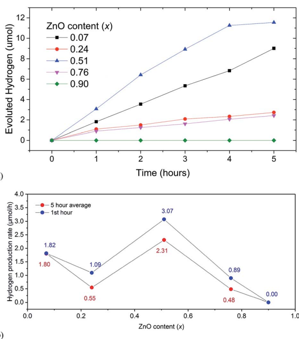
Fig. 5 (a) Hydrogen evolution for (GaN) 1-x (ZnO) x solid solution members for 5 hours. (b) Hydrogen evolution rates for first hour (blue) and 5 hour average (red).
