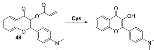
Scheme 44 An acrylate functionalised dimethylamino 3-hydroxyflavone fluorescent probe 48 . This system allowed for the ratiometric detection of Cys in human mesenchymal stem cells (hMSCs). Measurement conditions: PBS/DMSO (7.5 : 2.5), pH = 7.4.
