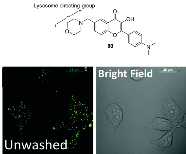
Fig. 9 A lysosomal-targeted ES IPT probe 80 that may be used for the imaging of lysosomes. Measurement conditions: n/a. Adapted with permission from ( J. Mater. Chem. B , 2018, 6 , 5050–5058). Copyright (2018) the Royal Society of Chemistry.
