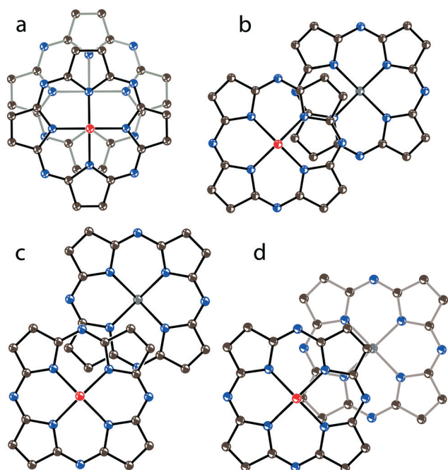
Fig. 12 View of the \pi -stacking \{Ti^{IV}O(Pc^{3-})\}^{2-}_2 dimers along the M=O bonds: (a) optimal overlapping observed in 1 , 8 and 13 ; (b) partial overlapping observed in 2 ; (c) weak overlapping observed in 4 and 9 ; (d) intermediate overlapping in 12 . Only 24-atom Pc planes are shown.
