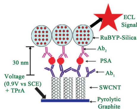
Fig. 11 Scheme of representation of ECL-based SWCNT immunosensors after addition of PSA and [Ru-(bpy) 3 ] 2+ -silica-Ab 2 nanoparticles. (Reprinted with permission from ref. 63. Copyright 2009 Royal Chemical Society.)
