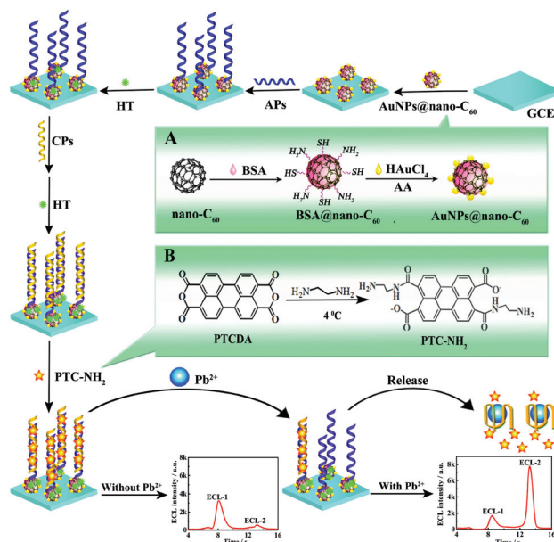
Fig. 22 Schematic illustration of the preparation process of the ratiometric aptasensor: inset of (A) and (B) display the preparation procedure of AuNPs@nano- \text{C}_{60} and PTC- \text{NH}_2 . (Reprinted with permission from ref. 14. Copyright 2015, American Chemical Society.)
