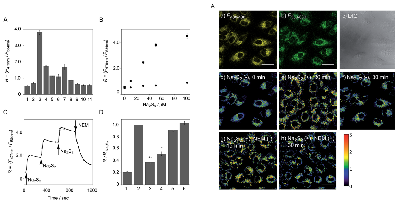
Fig. 3 (A) The ratio value ( R = F_{479 \text{ nm}}/F_{584 \text{ nm}} ) of 6 in the presence of various thiol species: (1) none, (2) Na 2 S (50 μM), (3) Na 2 S 2 (50 μM), (4) Na 2 S 4 (50 μM), (5) CysSSH (NOC7 (50 μM) + Na 2 S (50 μM) + L-Cys (50 μM)), (6) GSSH (NOC7 (50 μM) + Na 2 S (50 μM) + GSH (50 μM)), (7) mixture of NaOCl (50 μM) and Na 2 S (50 μM) in 0.1 M NaOH, (8) mixture of NaOCl (50 μM) and Na 2 S (50 μM) in 50 mM HEPES buffer (pH 7.4), (9) GSH (5 mM), (10) L-Cys (1 mM), (11) cystine (0.5 mM). Measurement conditions: [6] = 5 μM in 50 mM HEPES, 10 mM NaCl, 1 mM MgSO 4 , 0.4% Tween, pH 7.4, 25 °C. \lambda_{\text{ex}} = 410 nm. n = 3 . (B) Change in the fluorescence intensity ratio of 6 (5 μM) upon addition of Na 2 S 2 (0–100 μM, ■) and Na 2 S (0–100 μM, ●). n = 3 . (C) Time-trace plot of the ratio value ( R = F_{479 \text{ nm}}/F_{584 \text{ nm}} ) of 6 (5 μM) upon addition of Na 2 S 2 (30 μM at 30, 300, and 600 s) and N -ethylmaleimide (NEM, 500 μM at 900 s), n = 3 . (D) The reverse change of the ratio value ( R = F_{479 \text{ nm}}/F_{584 \text{ nm}} ) of 6 induced by the reactive species. Each bar represents R value of: (1) 6 (5 μM), (2) the hydropersulfide adduct of 6 (5 μM) with Na 2 S 2 (50 μM), (3) the adduct + NaOCl (100 μM), (4) the adduct + NEM (200 μM), (5) the adduct + GSH (5 mM), and (6) the adduct + L-Cys (1 mM). Measurement conditions: 50 mM HEPES, 10 mM NaCl, 1 mM MgSO 4 , 0.4% Tween, pH 7.4, 25 °C. \lambda_{\text{ex}} = 410 nm. n = 3 ; * P < 0.05 , ** P < 0.01 vs. hydropersulfide adduct of 6 with Na 2 S 2 (lane 2).
