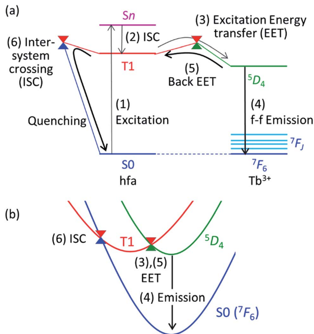
Fig. 2 Emission and quenching mechanisms of \text{Tb}^{3+} coordinated by hfa ligands shown in the Jablonski diagram (a) and the schematic potential energy surfaces (PESs) (b). S_n (or T_1 ) and 25+1L_J represent the electronic states of hfa and \text{Tb}^{3+} , respectively.
