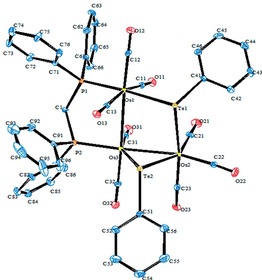
Fig. 7 Crystal structure of [\text{Os}_3(\mu\text{-TePh})_2(\text{CO})_8(\mu\text{-dppm})] (redrawn from ref. 116).
