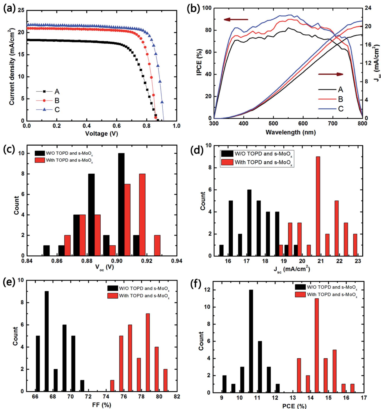
Fig. 2 Photovoltaic performance of devices. (a) J-V curves for devices (A–C) at reversed scan, under one sun illumination of AM1.5G, 100 \text{ mW cm}^{-2} (b) IPCE spectra (left) with integrated J_{sc} (right) based on IPCE measurement. Distribution histograms of V_{oc} (c), J_{sc} (d), FF (e), and PCE (f) of the 28 independently fabricated devices.
