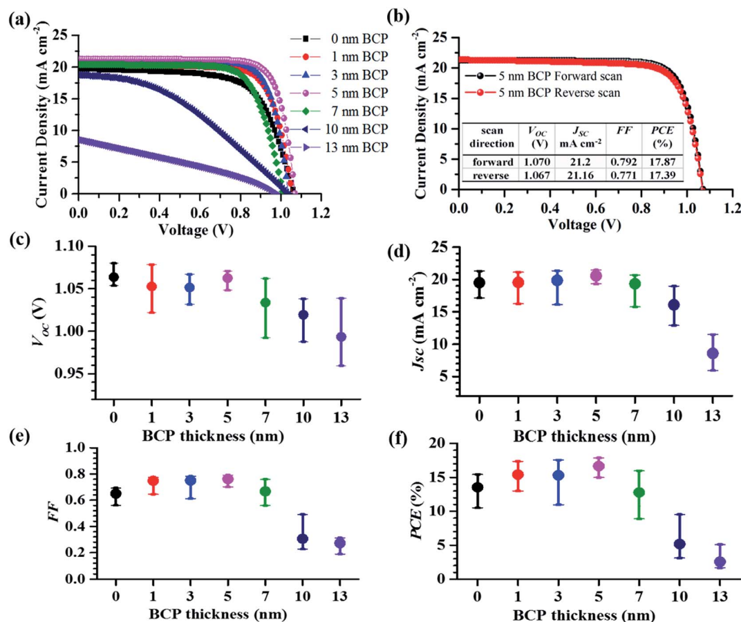
Fig. 2 (a) The forward scan J - V curves of PSCs with varying BCP layer thicknesses, measured under simulated solar light (AM 1.5G, 100 \text{mW cm}^{-2} ). (b) J - V curves of the champion device with a BCP layer thickness of 5 nm. Dependences of (c) open-circuit voltage ( V_{OC} ), (d) short-circuit photocurrent density ( J_{SC} ), (e) fill factor (FF), (f) PCE on the corresponding thickness of BCP layer, 10 samples being included.
