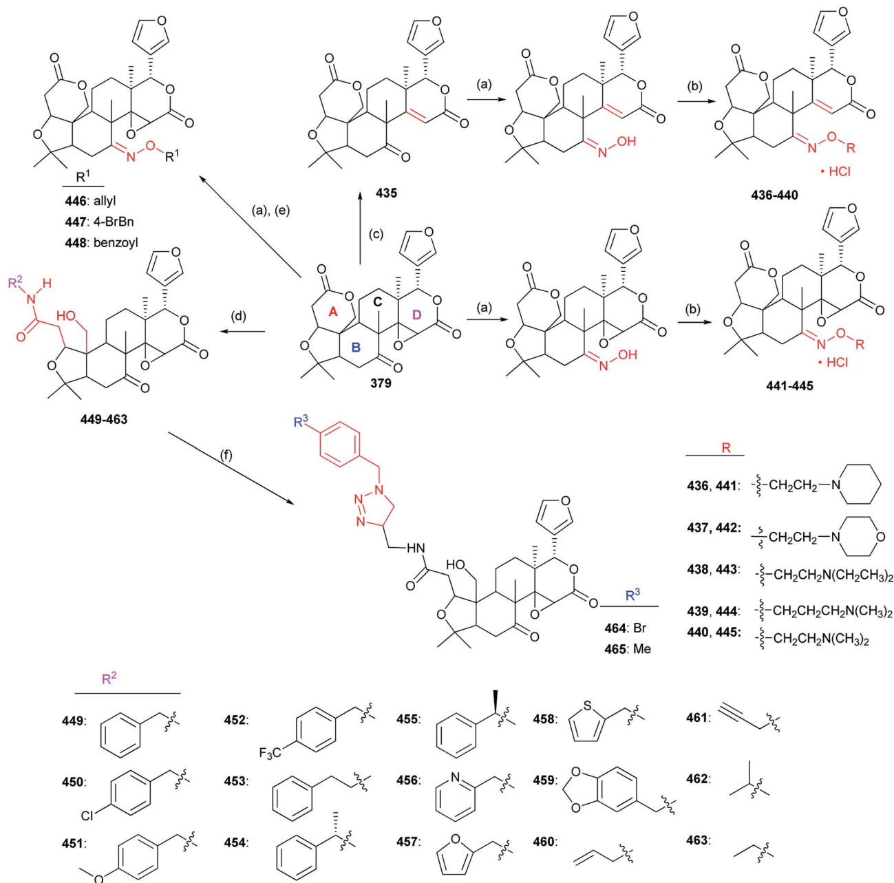
Scheme 7 Semisynthesis of limonin derivatives. Reagents and conditions: (a) \text{NH}_2\text{OH} \cdot \text{HCl} , pyridine, EtOH, reflux; (b) (i) \text{RCl} , \text{NaOH} , TBAB, dry THF, 80 °C; (ii) \text{HCl} , dry ether, \text{CH}_2\text{Cl}_2 ; (c) \text{HI} , \text{HOAc} ; (d) condition (i): abs. EtOH, appropriate amine, montmorillonite K-10, microwave-assisted; condition (ii): abs. EtOH, appropriate amine, montmorillonite K-10, reflux; condition (iii): \text{CH}_2\text{Cl}_2 , appropriate amine, montmorillonite K-10, ultrasonic bath; (e) \text{R}^1\text{Br} or \text{R}^1\text{Cl} , \text{NaH} , DMF, 0 °C to r.t.; (f) for 461, sodium ascorbate, \text{Cu}(\text{OAc})_2 \cdot \text{H}_2\text{O} , THF : \text{H}_2\text{O} (1 : 1), 1-(azidomethylene)-4-bromobenzene or 1-(azidomethylene)-4-methylbenzene, r.t., 10 h.
