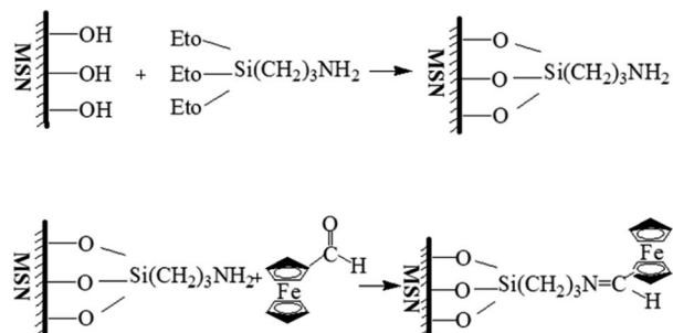
Scheme 2 Synthetic route of the MSN-Fc.
