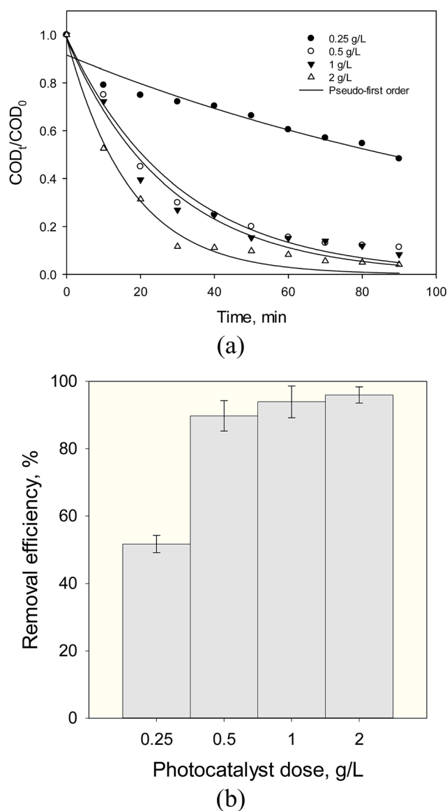
Fig. 10 (a) Kinetic curves, (b) removal efficiency of SMW with Fe_3O_4@TiO_2 (FT1) at different photocatalyst dose ( pH = 3 , 920\text{ mg L}^{-1} initial COD, 90 min reaction time and 30\text{ }^\circ\text{C} ).
