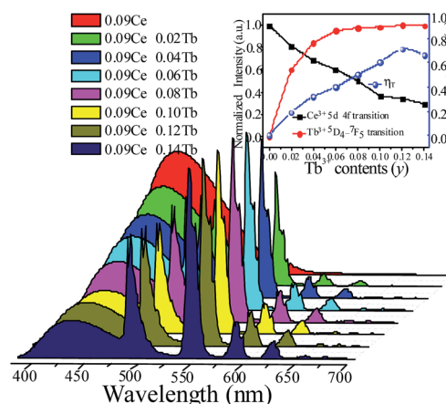
Fig. 7 PL spectra for LSN:0.09Ce 3+ , y Tb 3+ phosphors on Tb 3+ doping content ( y ) excited at 360 nm. The inset shows the emission intensity of Ce 3+ and Tb 3+ with different Tb 3+ contents, and energy transfer efficiency on changing Tb 3+ contents.
