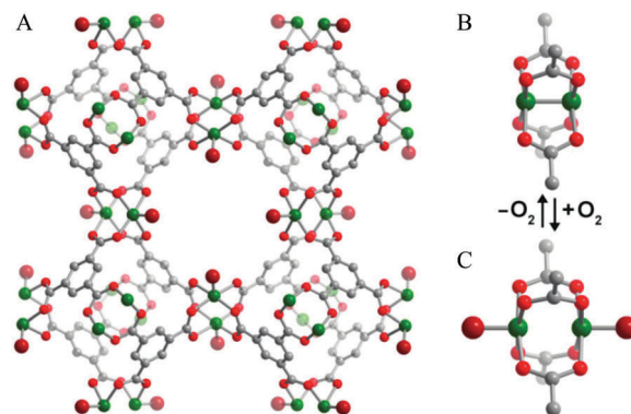
Fig. 8 (A) View of structure of [\text{Cr}_3(\text{BTC})_2] with adsorbed \text{O}_2 at the open Cr(II) sites. Rietveld refinements of NPD data revealed that the Cr–Cr distance lengthens from 2.06(2) \text{ Å} in the activated form (B) to 2.8 \text{ Å} in (C) upon coordination of \text{O}_2 . Colour scheme: Cr, green; O, red; C, grey. Reproduced from ref. 20 with permission from the American Chemical Society.
