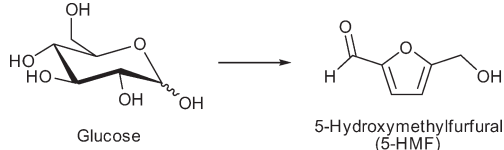
Scheme 4 Conversion of glucose to 5-HMF.
