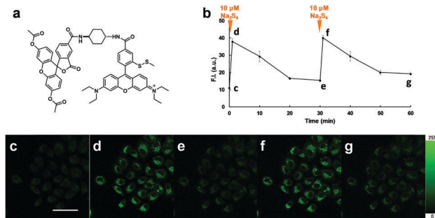
Fig. 4 (a) Chemical structure of SSip-1 DA. (b) Fluorescence intensity change of A549 cells loaded with SSip-1 DA upon repeated additions of 10 μM Na 2 S 4 . Data represent the mean ± SD ( n = 5). The mean fluorescence intensity of 5 cells is shown in the graph. (c–g) Fluorescence confocal microscopic images of A549 cells loaded with SSip-1 DA upon repeated additions of 10 μM Na 2 S 4 . Scale bar: 75 μm.
