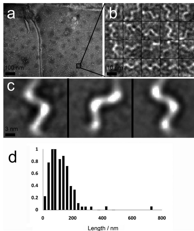
Fig. 4 (a) Contrast-enhanced TEM image showing numerous hydrogel fibrils with a twisted or helical appearance (scale bar 100 nm). (b) TEM image of a selection of twists/helical repeats in hydrogel fibrils (scale bar 10 nm). (c) Projection averages of selected images from (b), demonstrating that these repeats are regular and consistent with a helical structure (scale bar 3 nm). (d) Length distribution (normalised to highest frequency, 18, n = 118 ) of fibrils within 10 mM peptide hydrogel samples.
