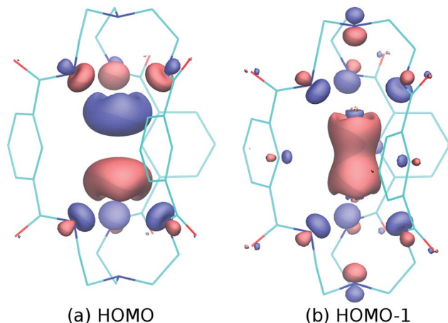
Fig. 2 HOMO (a) and HOMO–1 (b) of the model dianion [Sn_2(mBDCA-5t)]^{2-} based on the crystallographic coordinates of 1 and computed using ORCA 19 at the double-hybrid level of DFT theory 20 B2PLYP-D3/def2-TZVPP with corrections for dispersion 21 and including scalar relativistic effects via the ZORA method. 22
