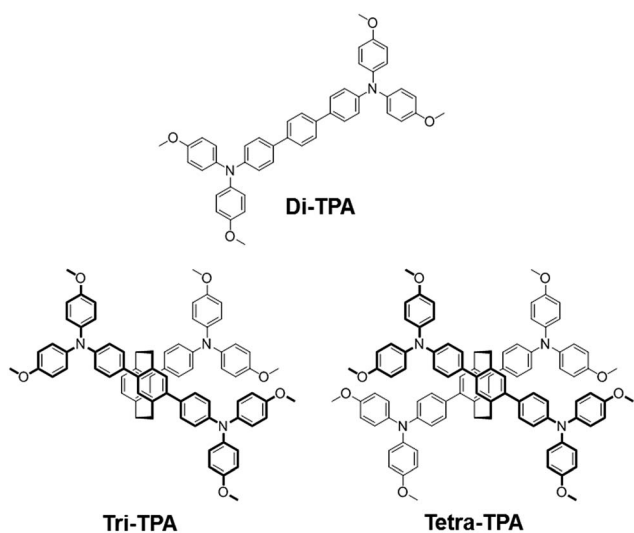
Fig. 1 Structures of HTMs containing two, three and four TPAs incorporated into a [2,2]paracyclophane core.
