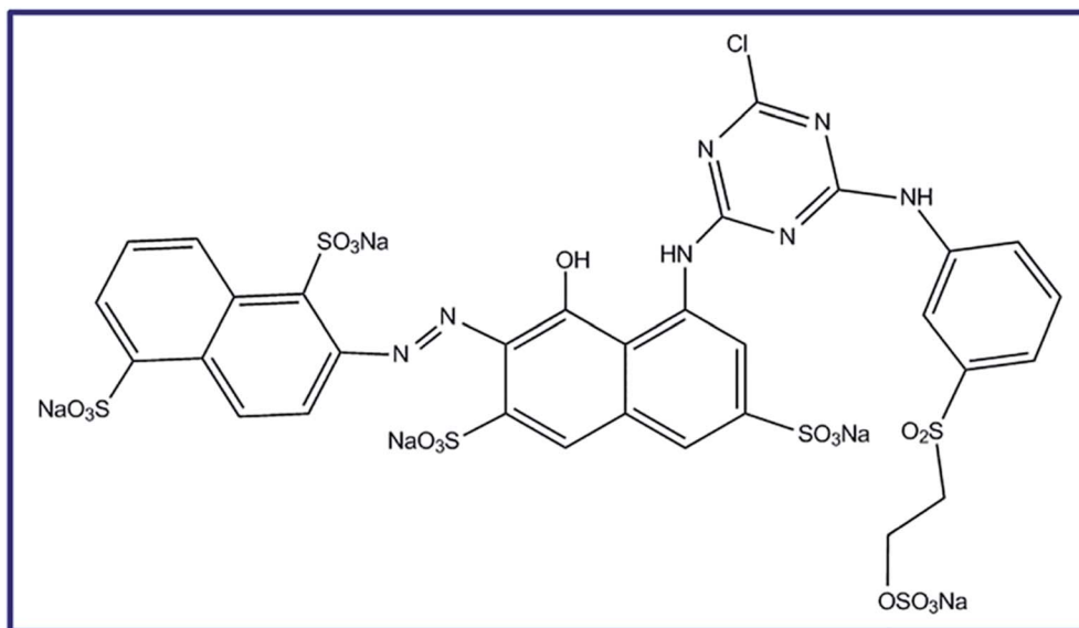
Scheme 1 Reactive Red 195 (RR195) dye molecular structure.
