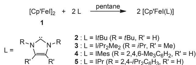
Scheme 1 Preparation of NHC-adducts to [\text{Cp}'\text{FeI}]_2 .
