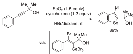
Scheme 41 Benzoselenophene synthesis through alkyne selenobromination/intramolecular S E Ar reaction.
