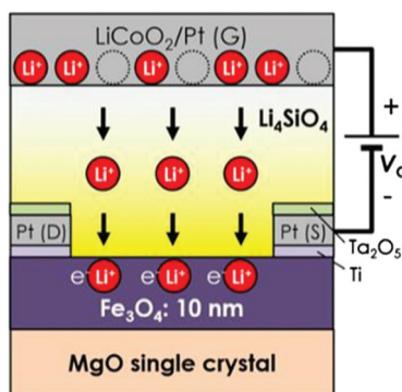
Fig. 7 A magnetic device whose magnetization and magnetoresistance can be controlled by injecting and withdrawing \text{Li}^+ ions to and from \text{Fe}_3\text{O}_4 . 23 Copyright (2016) American Chemical Society.
