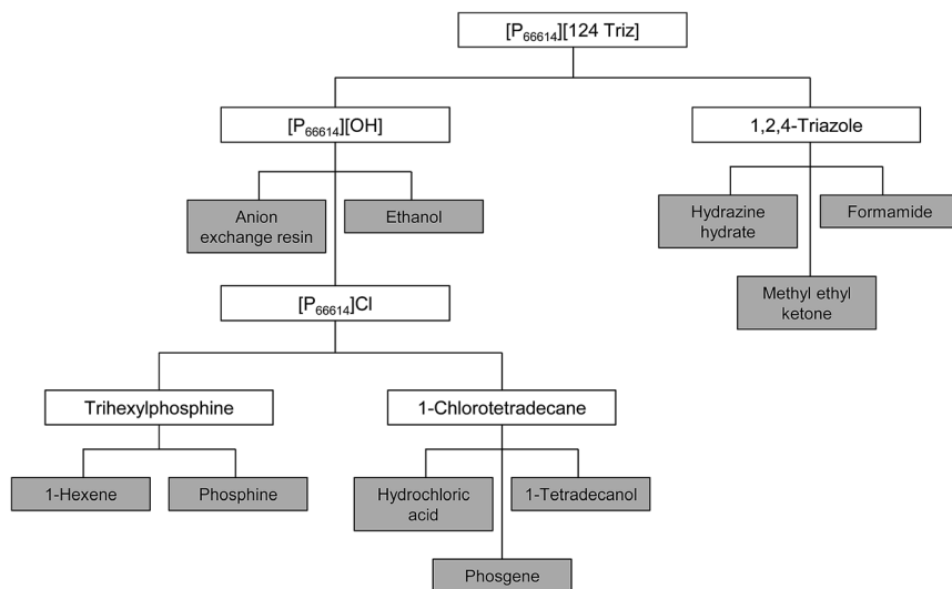
Fig. 3 The life cycle tree for the production of [P_{66614}][124\text{Triz}] (the shaded boxes indicate the compounds for which data are available in LCA databases. Data for the compounds shown in clear boxes are not available).
