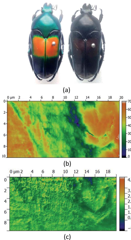
Fig. 7 (b) AFM topography and (c) \lambda = 10.21\ \mu\text{m} s-SNOM scattered amplitude image of a "natural photonic crystal", i.e. the shell of an iridescent beetle (a) that has in-built periodic structure that gives it a chiral light scattering characteristic which means its shell markings only show up under circularly polarised light. The s-SNOM image has given the chemical contrast of the components that make up the multilayers in the insect shell. In order to generate the shell's interference features in the visible part of the spectrum, the concentrations of these components vary on a sub-micron length scale, and only the s-SNOM can deliver chemical images at this resolution.
