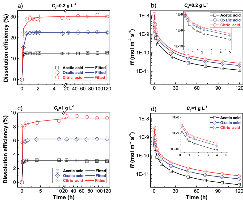
Fig. 1 Dissolution efficiency (%) and dissolution rate ( R ; \text{mol m}^{-2} \text{ s}^{-1} ) of HANPs as a function of time under different LMWOAs (1 mM acetic acid, oxalic acid, and citric acid, respectively) in batch experiments at initial HANPs concentrations ( C_0 ) of 0.2 \text{ g L}^{-1} (a and b) and 1 \text{ g L}^{-1} (c and d), respectively. Error bars represent the standard deviations in triplicate experiments. Insets in (b) and (d) highlight R change during the early stages where y-axes are shown in logarithmic scale.
