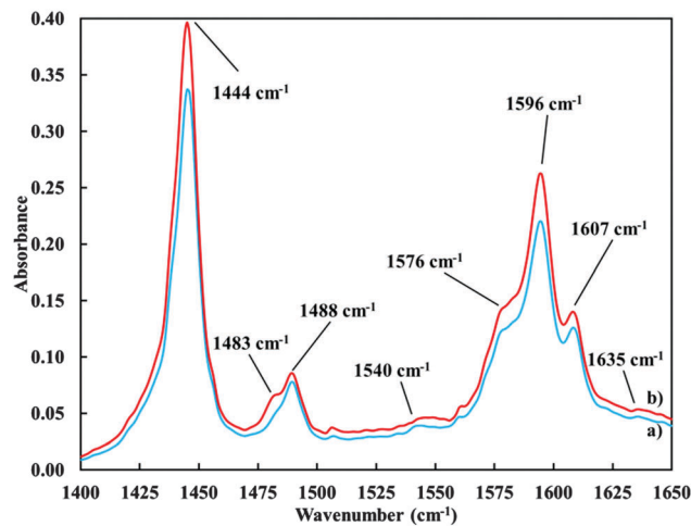
Fig. 6 FT-IR spectra of catalyst material B under pyridine saturated nitrogen flow at 200 °C cell temperature after (a) 5 min and (b) after 30 min. The catalyst material was pre-treated with ethanol saturated nitrogen flow at 200 °C in situ cell temperature for 30 min before switching to pyridine atmosphere.
