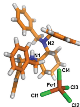
Fig. 1 Stick model of the asymmetric unit of [\text{LH}]^+ \cdot [\text{FeCl}_4]^- ( \alpha -phase). Color code: carbon: orange; nitrogen: blue; chloride: green; iron: brown; hydrogen: white.
