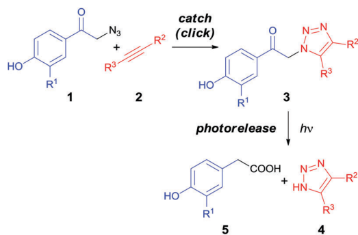
Scheme 1 A "catch and photorelease" strategy.
