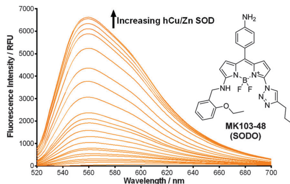
Fig. 1 Chemical structure and fluorescence spectra of SODO (10 \mu\text{M} ) after incubation with serial concentrations of hCu/Zn-SOD from 0.01 to 5 \text{mg mL}^{-1} in 20 mM Tris-HCl buffer (pH = 7.4). \lambda_{\text{exc}} : 460 nm. \Phi_{\text{F}} in hCu/Zn-SOD: 0.45.
