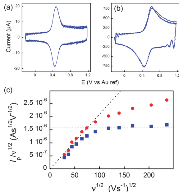
Fig. 7 (a and b) Voltammograms of C 60 Fc at 836 (a) and 55 850 \text{V s}^{-1} (b) in acetonitrile + 1 M tetra- n -butylammonium tetrafluoroborate. (c) Peak current evolution with the scan rate. Red dots: experimental data. Blue dots: corrected data featuring a diffusion plateau at large scan rates. Adapted from ref. 62.
