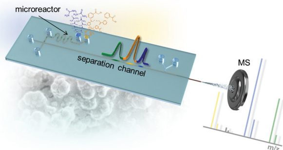
Fig. 2 Microfluidic layout of the chip with integrated serpentine micro-reactor structure, electrochromatographic separation column and electrospray ionization tip leading into a mass spectrometer.
