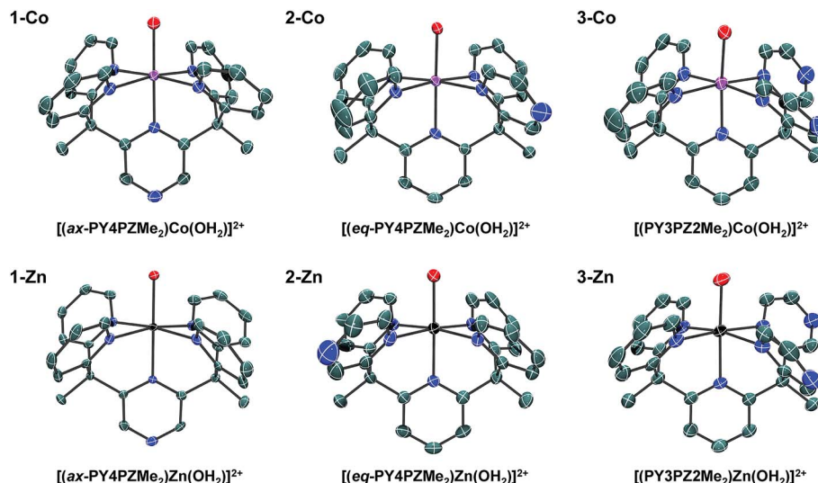
Fig. 2 Crystal structures of cations in the following salts: 1-Co, [(ax-PY4PZMe_2)Co(OH_2)](OTf)_2 ; 2-Co, [(eq-PY4PZMe_2)Co(OH_2)](OTf)_2 ; 3-Co, [(PY3PZ2Me_2)Co(OH_2)](OTf)_2 ; 1-Zn, [(ax-PY4PZMe_2)Zn(OH_2)](OTf)_2 ; 2-Zn, [(eq-PY4PZMe_2)Zn(OH_2)](OTf)_2 ; 3-Zn, [(PY3PZ2Me_2)Zn(OH_2)](OTf)_2 . Thermal ellipsoids are drawn at the 70% probability level. Hydrogen atoms have been omitted for clarity.
