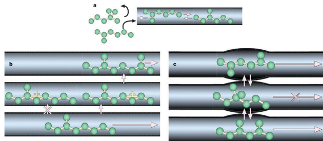
Fig. 1 Different types of shape selectivity in zeolites. (a) Reactant shape selectivity: molecules that are too large to enter the zeolite pores cannot reach acid sites for reaction and are therefore not converted into products. (b) Transition state shape selectivity: molecules (and transition states) that are too large to fit inside a pore do not form. (c) Product shape selectivity: new molecules are formed in the adsorbed phase, but are too large to desorb as a product. (Reprinted from ref. 4 with permission, Copyright Nature Publishing Group.)
