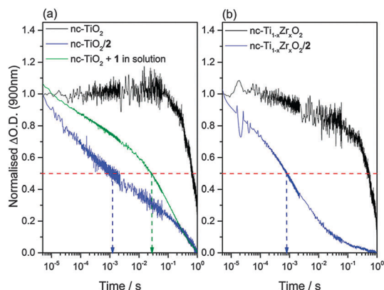
Fig. 5 Transient absorption decays of (a) unmodified \text{TiO}_2 (black), \text{TiO}_2\text{-2} (blue) and \text{TiO}_2 with 1 \times 10^{-4} M in solution (green) and (b) \text{Ti}_{1-x}\text{ZrO}_2 (black) and \text{Ti}_{1-x}\text{ZrO}_2\text{-2} (blue) measured in \text{CH}_3\text{CN} with 0.1 M TEOA. The samples were excited at 355 nm ( 350 \mu\text{J cm}^{-2} ) and probed at 900 nm. The samples were purged under \text{N}_2 for 15 min prior to measurements. A useful measure for the kinetics of the process is t_{50\%} (dotted lines), which represents the time delay by which the yield of photoelectrons has dropped by 50% when compared to an initial concentration, here defined to be the photoelectron yield at 4 microseconds.
