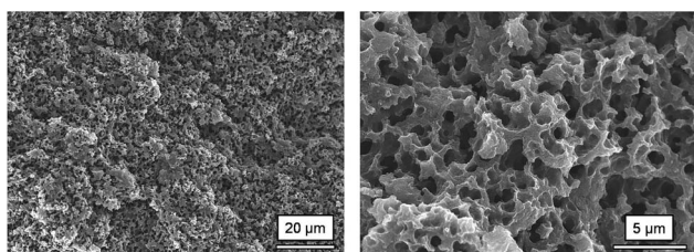
Fig. 3 SEM micrographs of the CDC monoliths.
