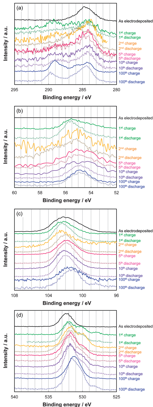
Fig. 12 XPS spectra of C_{1s} (a), Li_{1s} (b), Si_{2p3/2} (c), and O_{1s} (d) on the Si–O–C composite film and Li–Si–O–C composite anodes after the 1st charge, 1st discharge, 2nd charge, 2nd discharge, 5th charge, 5th discharge, 10th charge, 10th discharge, 100th charge, and 100th discharge. All spectra were corrected based on the C–C bond at 284 eV after peak separation of the C_{1s} spectra into C–C, C–O, and C=O peaks. The baselines of each graph are displaced for clarity. Reproduced from data published in ref. 37.
