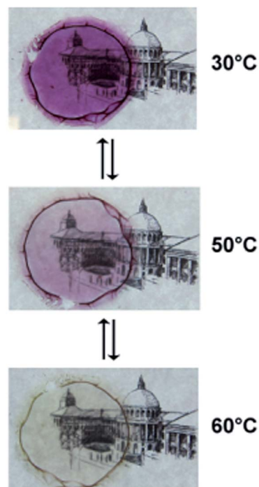
Fig. 7 Photographs of a thermochromic film of [\text{Fe}(\text{NH}_2\text{trz})_3](2\text{ns})_2 prepared from a gel of type B at c_{\text{Fe}} = 0.0371 M and \text{NH}_2\text{trz}/\text{Fe}^{2+} 3 : 1 at 30 °C, 50 °C and 60 °C.
