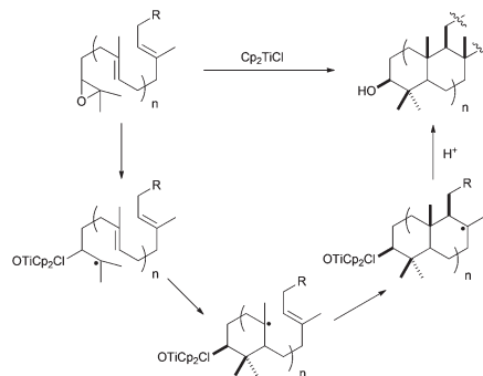
Scheme 29 Example of \text{Cp}_2\text{TiCl} mediated epoxypolyprene cyclisation.
